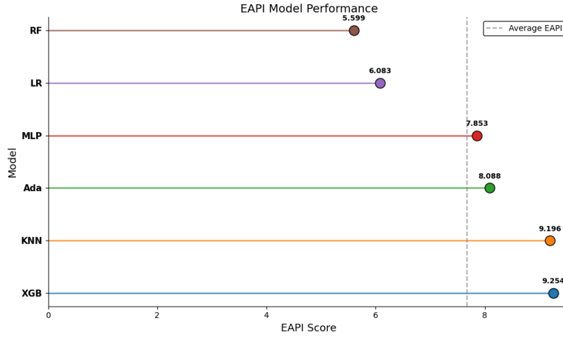
(b) EAPI scores
