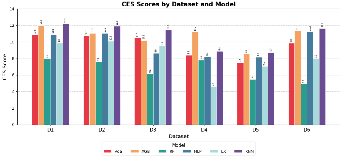
(a) Dataset wise CES scores per model
