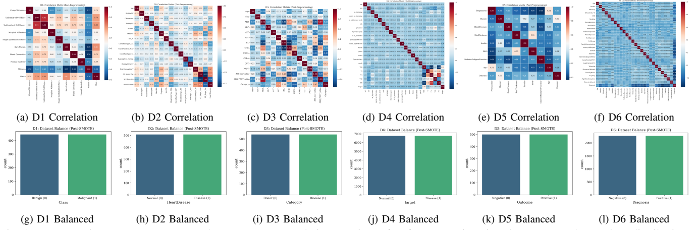
Fig. 1: Preprocessing summary: top row shows Pearson correlation matrices after feature engineering; bottom row shows class distributions after SMOTE balancing to a 1:1 ratio across all six datasets.
