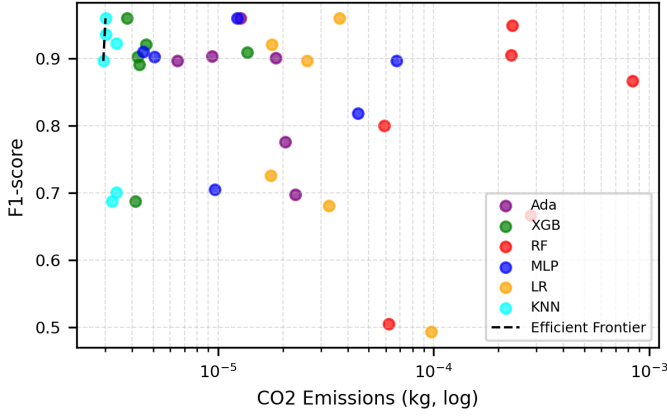
Fig. 3: Efficient frontier plot mapping F1-score against log-scaled CO 2 equivalent emissions. KNN and XGBoost models cluster near the optimal top-left frontier, while Random Forest remains a significant outlier.
